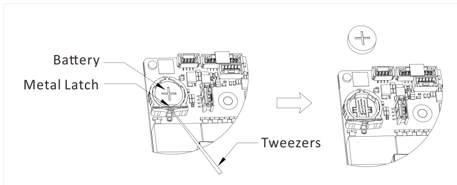
Figure 1-1 Remove Battery
