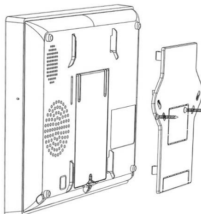
Plaque de suspension murale ×1 Vis ×2
